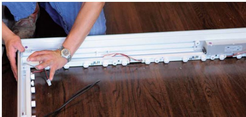
PERIMETER LIGHTING
