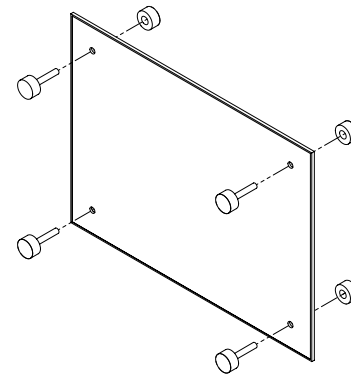
Installing standard standoffs with predrilled holes on the panel.
