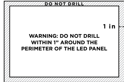
PANEL BACK VIEW
